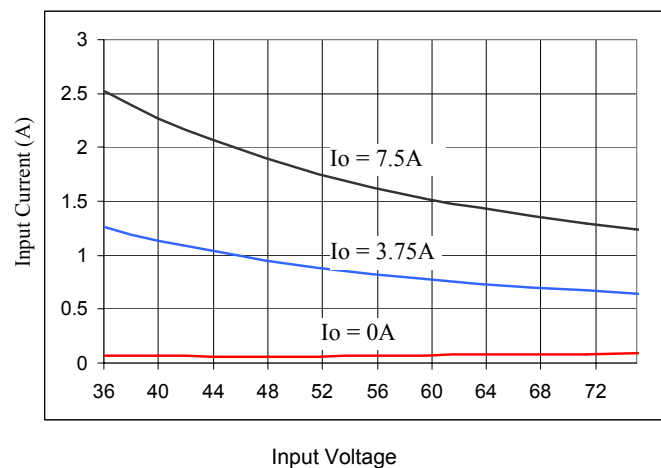
Figure 2. Input Characteristics
