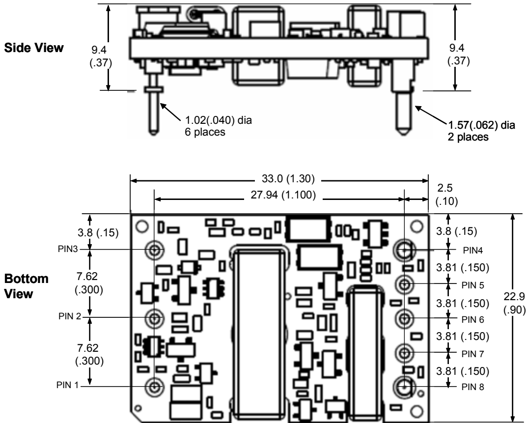
Figure 17. Open Frame Converter
