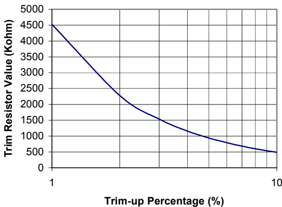
Figure 13. Trim-Up Resistor Selection
