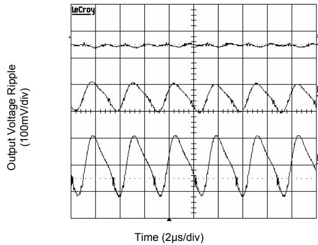
Figure 4. Output Ripple Voltage at 7.5A Load
