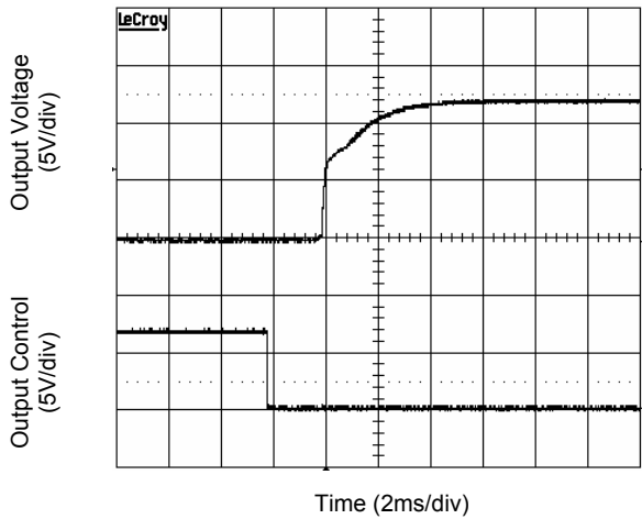
Figure 3. Start-Up from Enable Control Input voltage 48V, Output current 7.5A)
