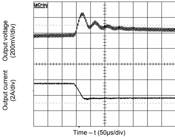
Figure 5. Transient Load Response ( V_{in} = 48V ; I_o changes from 3.75A to 5.63A; Slew rate 0.1A/ \mu s )
