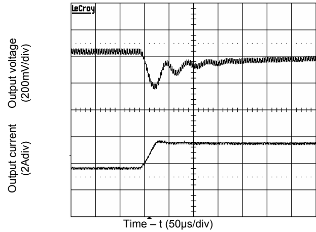
Figure 6 Transient Load Response ( V_{in} = 48V ; I_o changes from 5.63A to 3.75A; Slew rate 0.1A/ \mu s )
