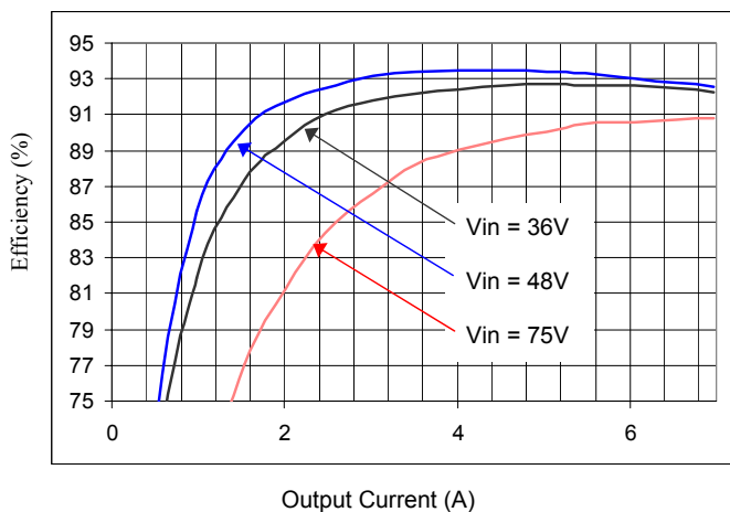
Figure 1. Efficiency vs. Load Current (25°C)
