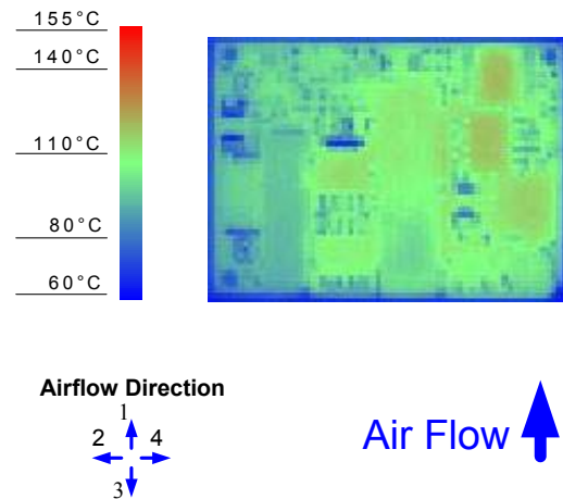
Figure 8. Thermal Image for Airflow Direction 1 (4.2A output, 70°C ambient, natural convection, V_{in} = 48V , open frame soldering interface)
