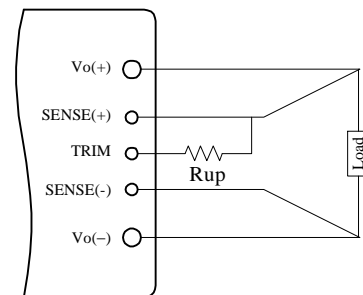
Figure 21 Circuit to Increase Output Voltage
