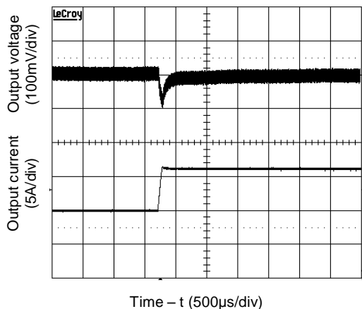
Figure 7. Transient Load Response ( V_{in} = 48V ; I_o changes from 15A to 22.5A; Slew rate 0.1A/ \mu s )
