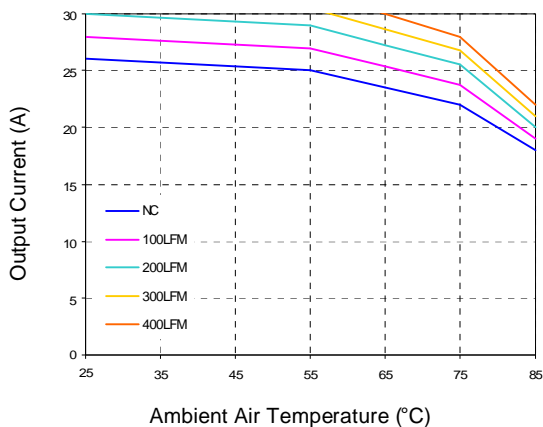
Figure 9. Current Derating Curve for Airflow Direction 3 (Referring to Figure 10 for Airflow Direction; V_{in} = 48V ; open frame; soldering interface)
