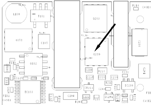
Figure 22. Temperature Monitoring Location
