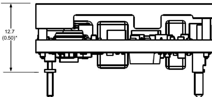
Figure 24. Converter with a Baseplate
