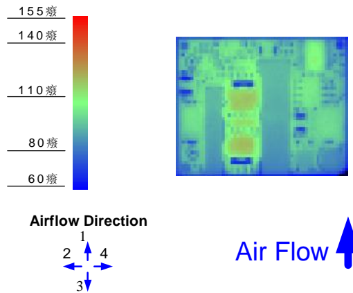
Figure 10. Thermal Image for Airflow Direction 1 ( V_{in} = 48V , 29A output, 55°C ambient, 200 LFM, open frame; soldering interface)
