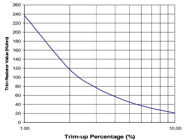
Figure 19 Trim-Up Resistor Selection
