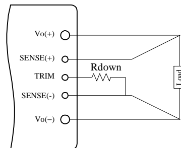
Figure 20 Circuit to Decrease Output Voltage
