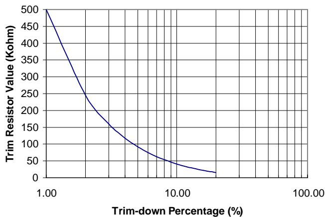
Figure 18 Trim-Down Resistor Selection
