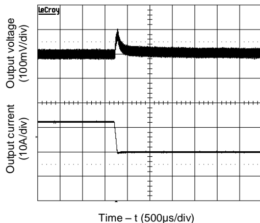
Figure 8. Transient Load Response ( V_{in} = 48V ; I_o changes from 22.5A to 15A; Slew rate 0.1A/ \mu s )
