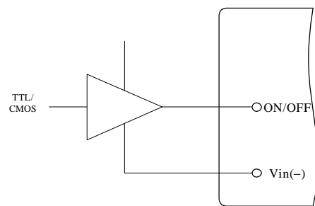
Figure 17 Direct Logic Drive
