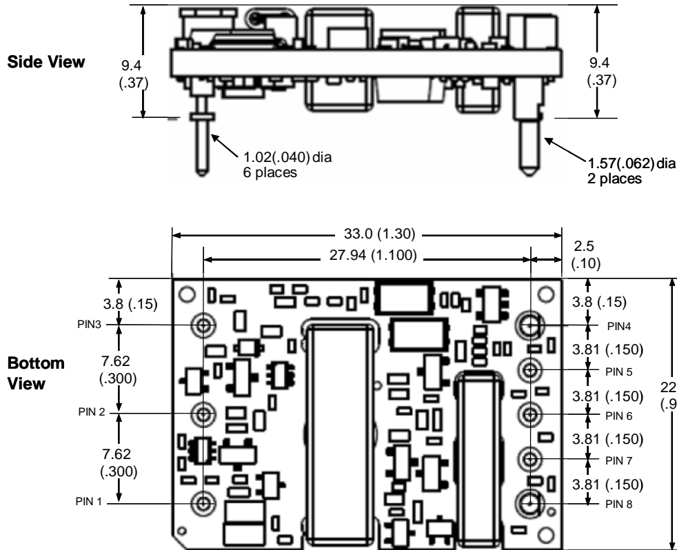
Figure 23. Open Frame Converter
