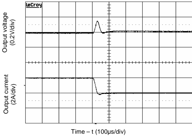
Figure 5. Transient Load Response (Vin= 24V; Io changes from 75% to 50%; Slew rate 0.1A/µs)
