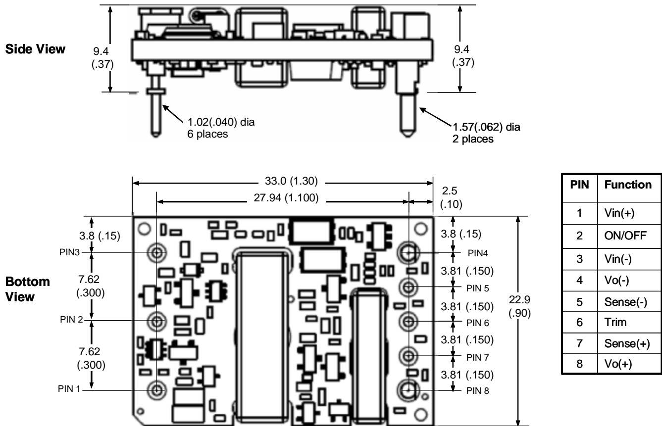
Figure 17. Open Frame Converter
