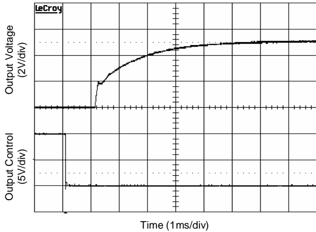
Figure 3. Start-Up from Enable Control Input voltage 24V, Output current 0A
