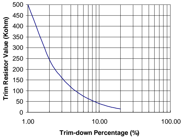
Figure 12. Trim-Down Resistor Selection
