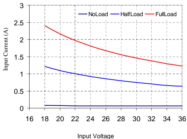
Figure 2. Input Characteristics
