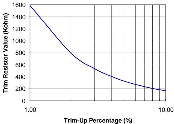
Figure 13. Trim-Up Resistor Selection
