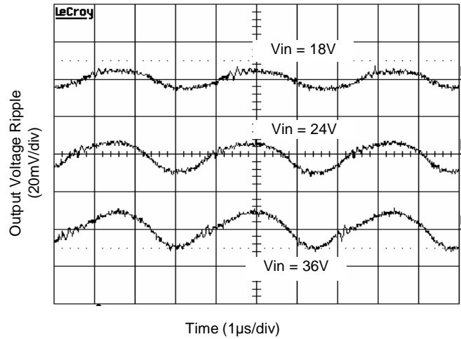
Figure 4. Output Ripple Voltage at 8A Load
