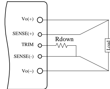
Figure 14. Circuit to Decrease Output Voltage
