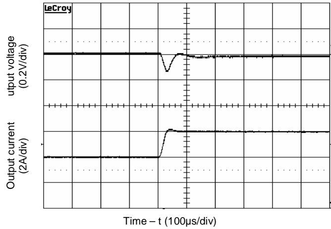
Figure 6 Transient Load Response (Vin= 24V; Io changes from 50% to 75%; Slew rate 0.1A/µs)
