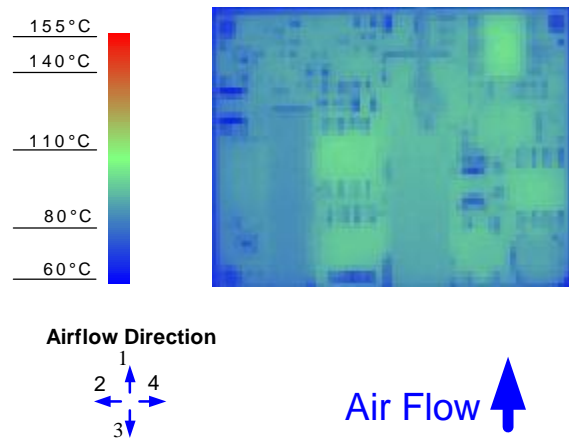
Figure 8. Thermal Image . (7.5A output, 85°C ambient, natural convection, Vin = 24V open frame soldering interface)
