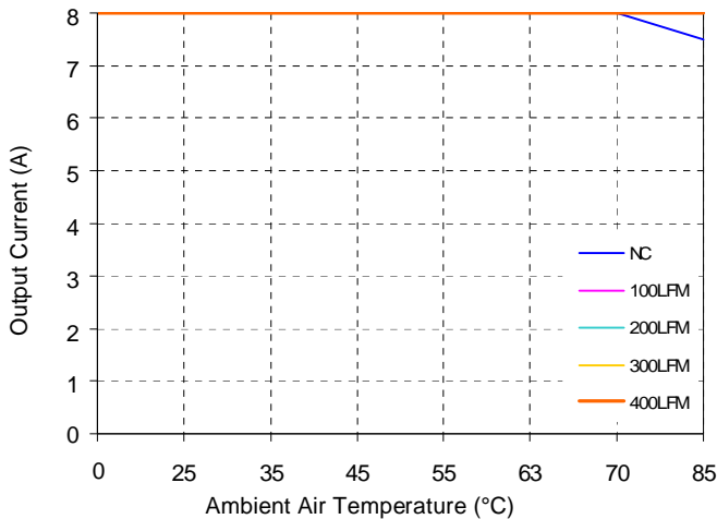
Figure 7. Current Derating Curve for Airflow Direction 1 ( Vin = 24V; open frame; soldering interface)
