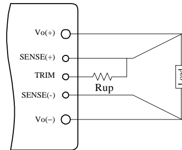
Figure 15. Circuit to Increase Output Voltage
