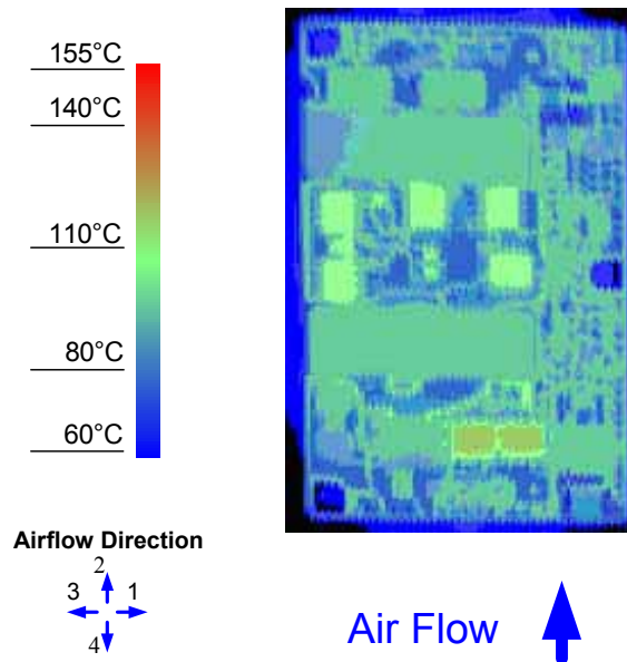
Figure 14. Thermal Image for Airflow Direction 2 (8.3A output, 55°C ambient, 200 LFM, Vin = 48V open frame unit using solder interface)
