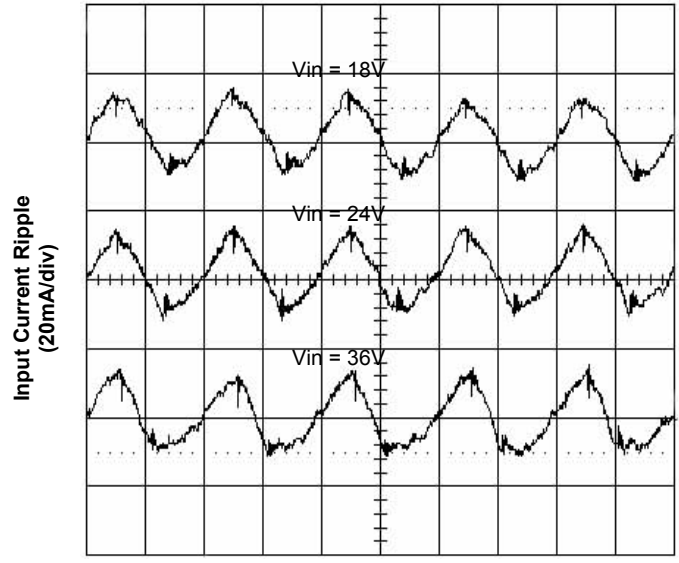
Time - t (2µs/div) Figure 6. Input Reflected Ripple Current at 10A Load
