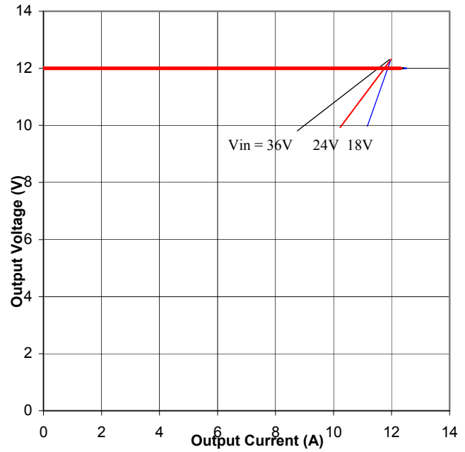
Figure 10. Output Characteristics
