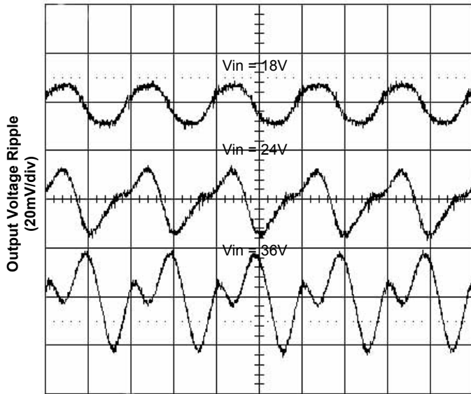
Time - t (2µs/div) Figure 5. Output Ripple Voltage at 10A Load
