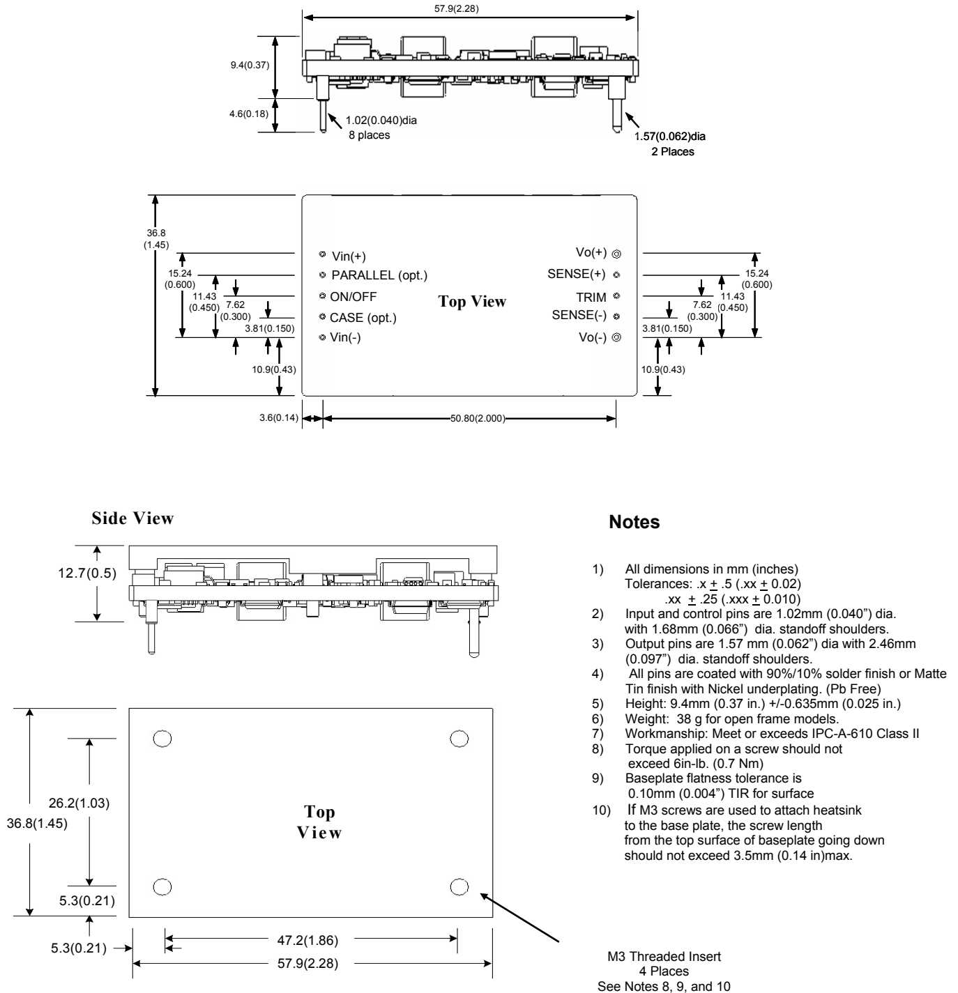
Figure 25. Converter with Optional Baseplate
