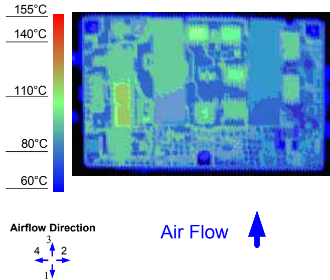
Figure 12. Thermal Image for Airflow Direction 3 (8.5A output, 55^{\circ}C ambient, 200 LFM, V_{in} = 48V open frame unit using socket interface)
