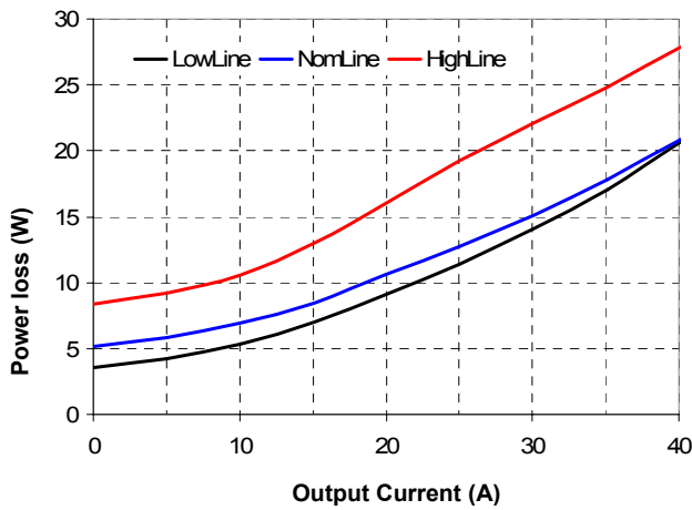
Figure 3. Power loss vs. Output Current
