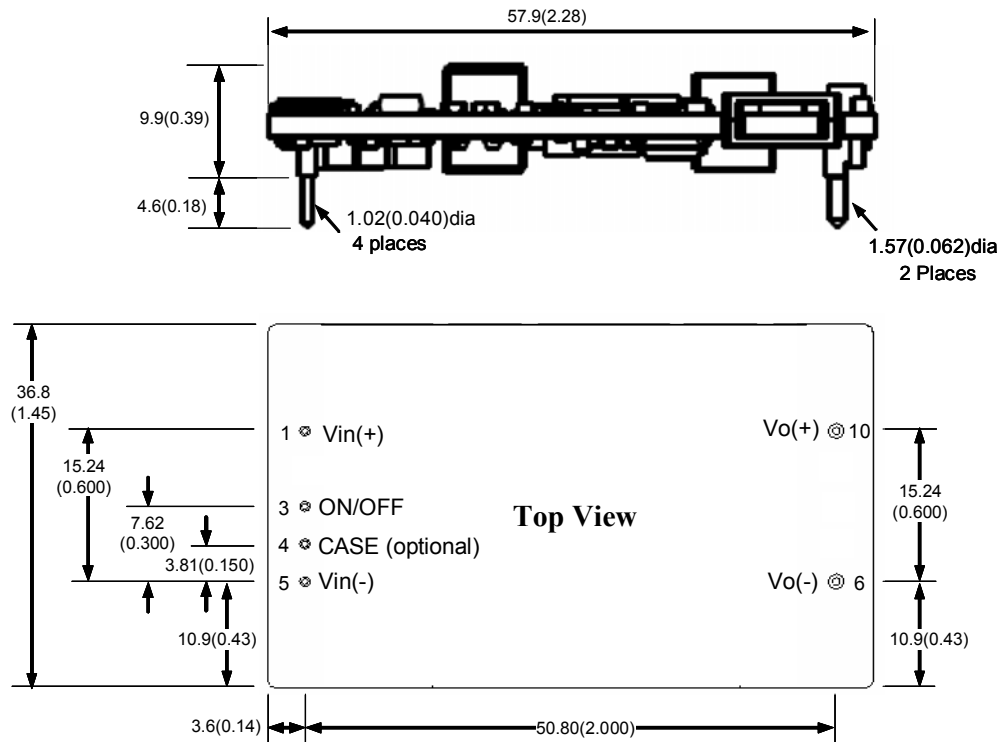
Figure 17. Open Frame Converter
