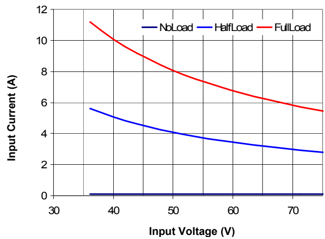
Figure 4. Input Characteristic
