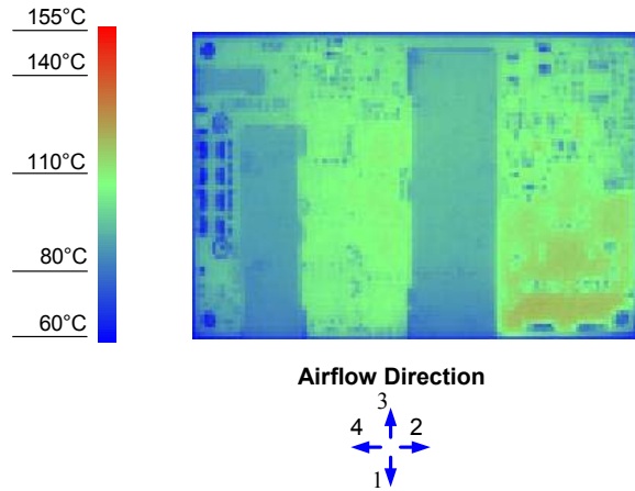
Figure 10. Thermal Image for Airflow Direction 3 (31A output, 55°C ambient, 200 LFM, Vin = 48V open frame unit )
