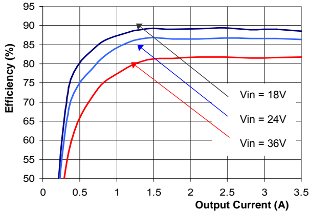
Figure 1(g). Efficiency vs. Load Current (25°C, 5V output)
