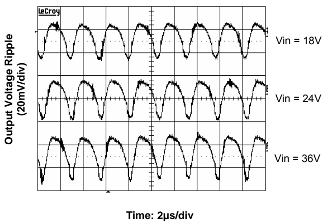
Figure 4. Output Ripple Voltage at 5V, 3.5A Output
