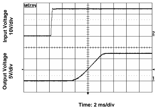
Figure 5. Start-Up from Application of Input Voltage Input voltage 24V, output current 3.5A, output voltage 12V.
