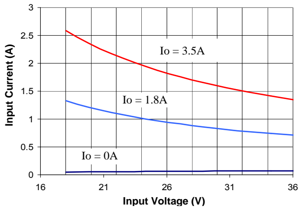
Figure 2. Input Characteristic (12V output)
