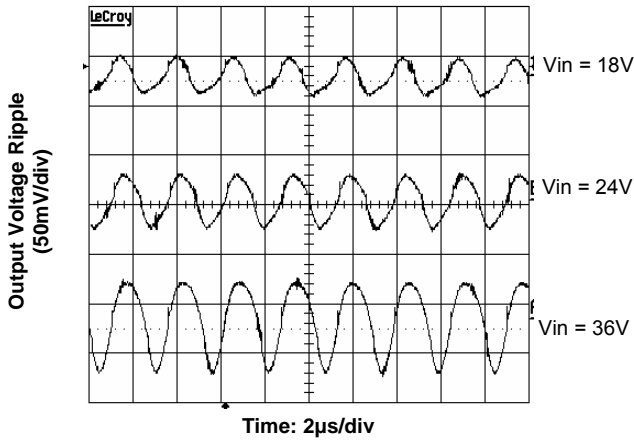
Figure 6. Output Ripple Voltage at 12V, 5A Output
