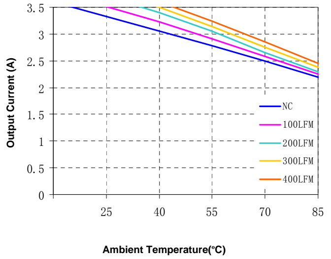
Figure 12(b). Current Derating Curve for 12V Output ( V_{in} = 24V open frame)
