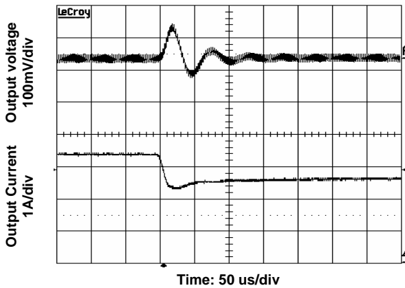
Figure 8. Transient Load Response Input/output voltage 24/12V, Output current 3.5A->1.65A, Slew rate 0.1A/µs.
