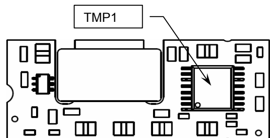
Figure 16. NBS3 Bottom View — Temperature Monitoring Point TMP1 for Thermal Shutdown
