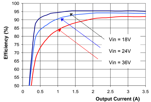
Figure 1(h). Efficiency vs. Load Current (25°C, 12V output)
