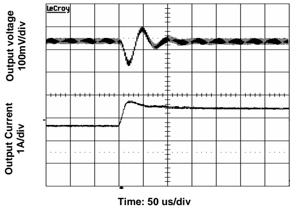
Figure 9. Transient Load Response Input/output voltage 24/12V, Output current 1.65A->3.5A, Slew rate 0.1A/µs .
