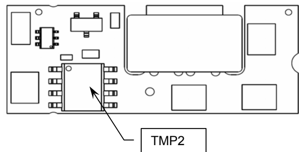
Figure 17. NBS3 Top View — Temperature Monitoring Point TMP2 for Derating Operation
