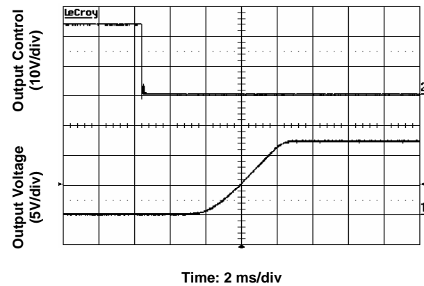
Figure 3. Start-Up from Enable Control Input voltage 24V, Output current 3.5A, output voltage 12V.
