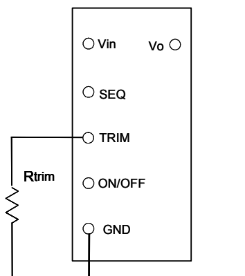
Figure 15 Circuit to Trim Output Voltage
