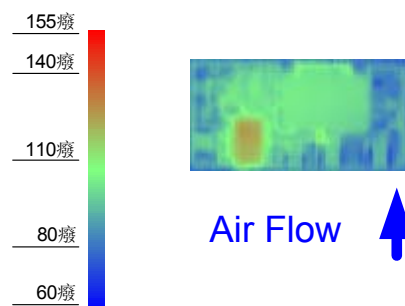
Figure 11. Thermal Image. V_{in} = 12V , 3.3V/6.5A output, 55°C ambient, 200 LFM
