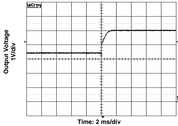
Figure 7. Start-Up with Prebias Input voltage 24V, Output current 0A, Output voltage 5V, Prebias 3.3V
