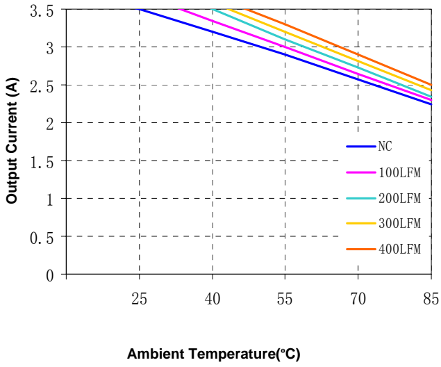
Figure 12(a). Current Derating Curve for 5V Output ( V_{in} = 24V open frame)
