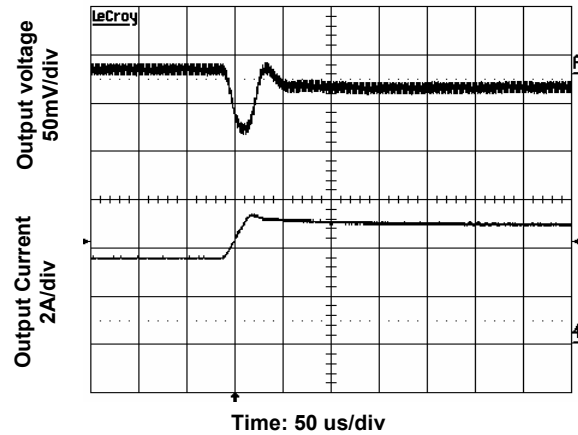
Figure 9. Transient Load Response Input/output voltage 24/12V, Output current 3.75A->5A, Slew rate 0.1A/µs .
