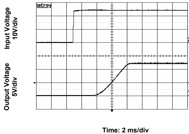
Figure 5. Start-Up from Application of Input Voltage Input voltage 24V, output current 5A, output voltage 12V.
