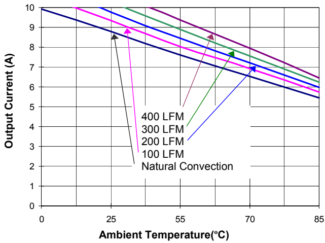
Figure 12(a). Current Derating Curve for 5V Output ( V_{in} = 24V open frame)
