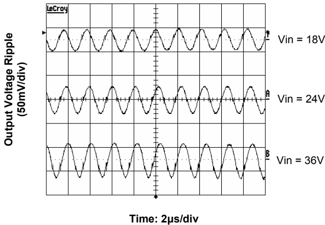
Figure 4. Output Ripple Voltage at 5V, 9A Output
