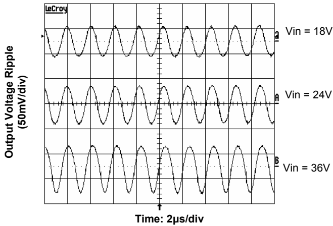
Figure 6. Output Ripple Voltage at 12V, 5A Output
