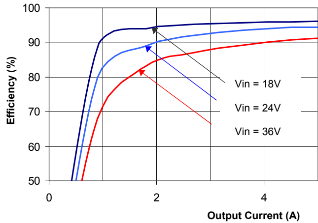
Figure 1(h). Efficiency vs. Load Current (25°C, 12V output)
