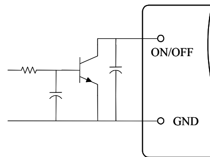
Figure 14. Open Collector Enable Circuit
