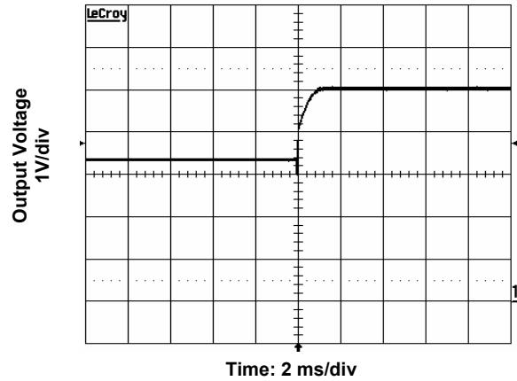
Figure 7. Start-Up with Prebias Input voltage 24V, Output current 0A, Output voltage 5V, Prebias 3.3V
