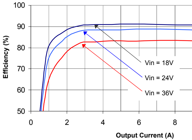
Figure 1(g). Efficiency vs. Load Current (25°C, 5V output)
