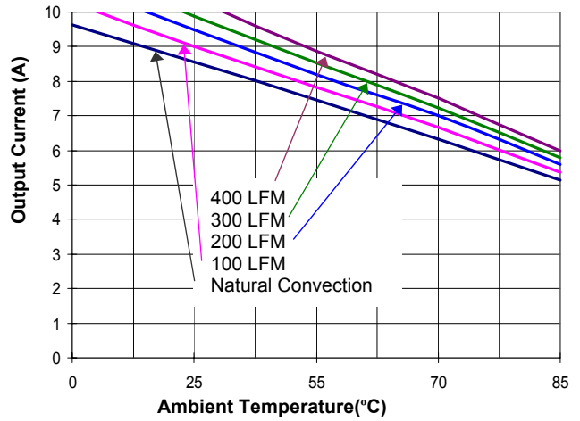
Figure 12(b). Current Derating Curve for 12V Output ( V_{in} = 24V open frame)
