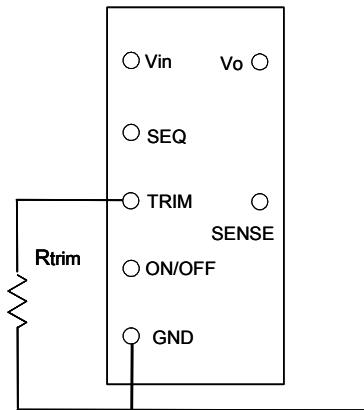
Fig. 16 Circuit to Trim Output Voltage
