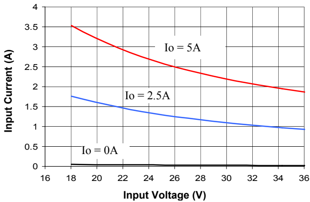
Figure 2. Input Characteristic (12V output)
