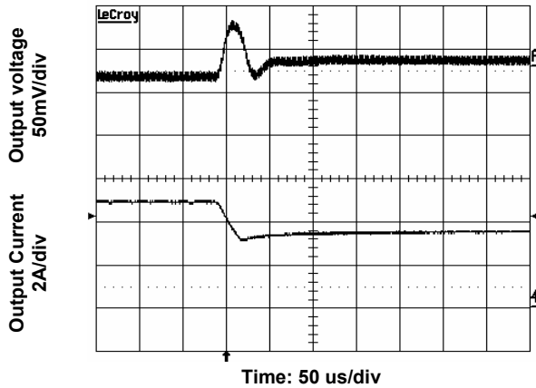
Figure 8. Transient Load Response Input/output voltage 24/12V, Output current 5A->3.75A, Slew rate 0.1A/µs.
