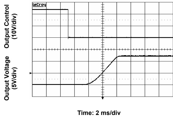
Figure 3. Start-Up from Enable Control Input voltage 24V, Output current 5A, output voltage 12V.
