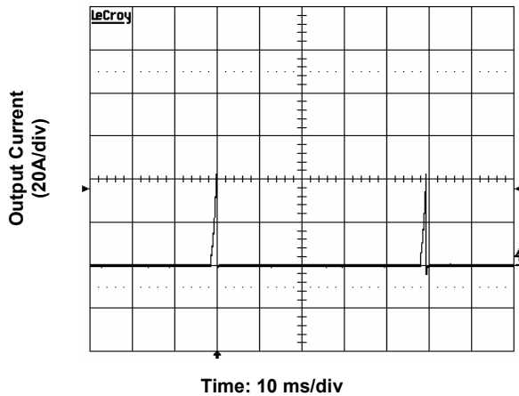
Figure 10. Short Circuit Current. V_{in} = 24V
