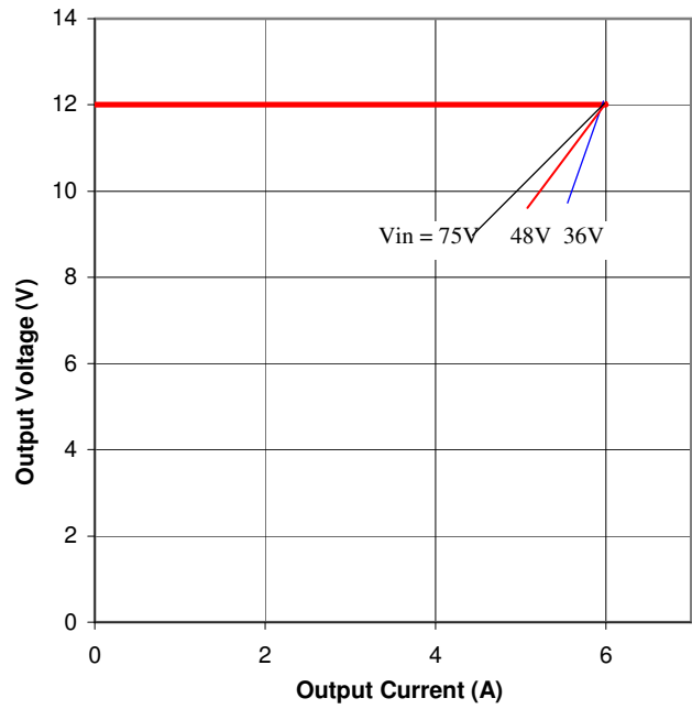
Figure 10. Output Characteristics
