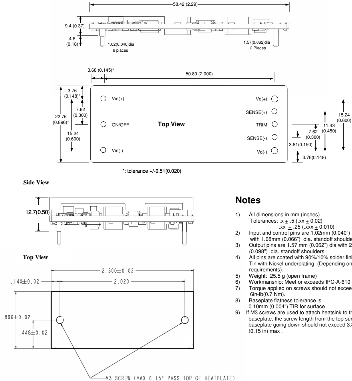
Figure 20. Converter with optional baseplate
