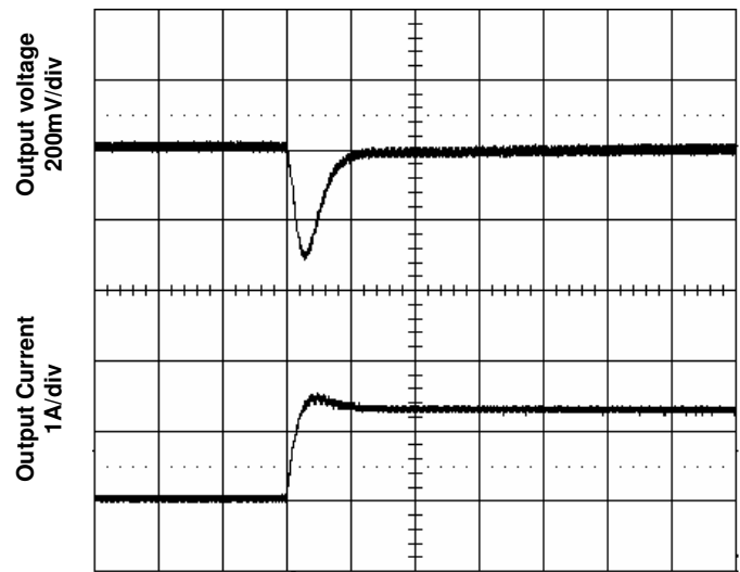
Figure 8. Transient Load Response
