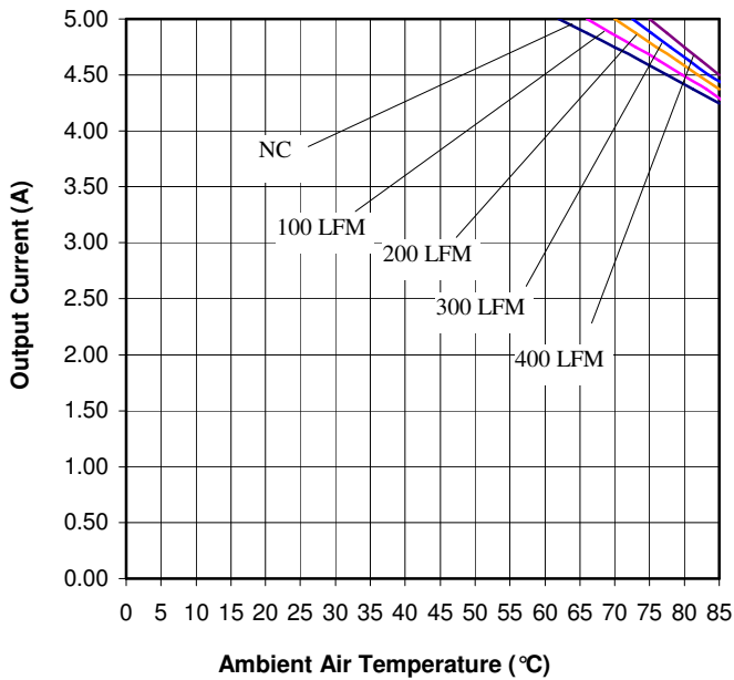
Figure 11. Current Derating Curve for Airflow Direction 3 (Ref. Fig. 12 for Airflow Direction; V_{in} = 48V open frame unit soldered into fixture board)
