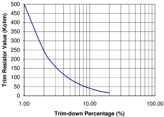
Fig. 18 Trim-Down Resistor Selection
