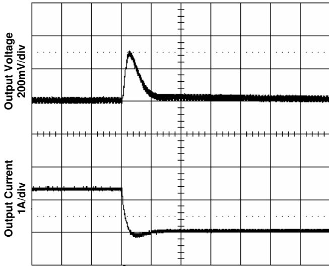
Figure 7. Transient Load Response
