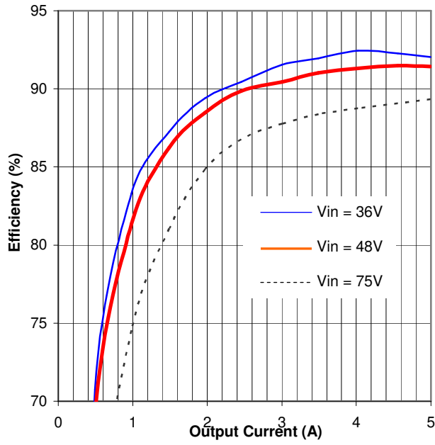
Figure 1. Efficiency vs. Load Current (25°C)
