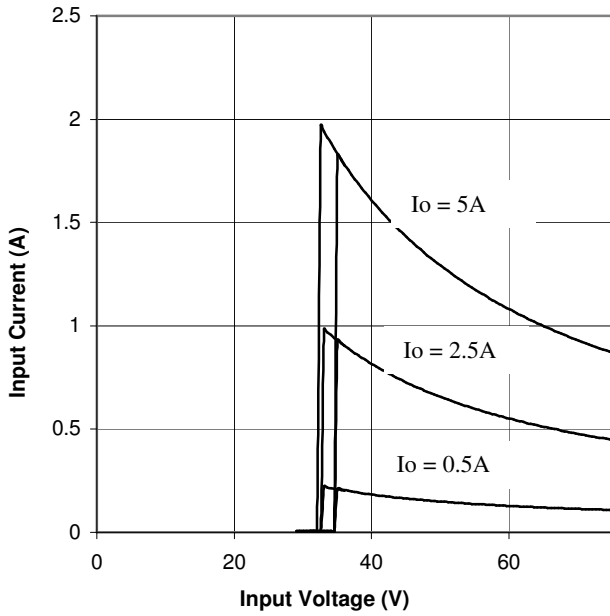
Figure 9. Input Characteristics
