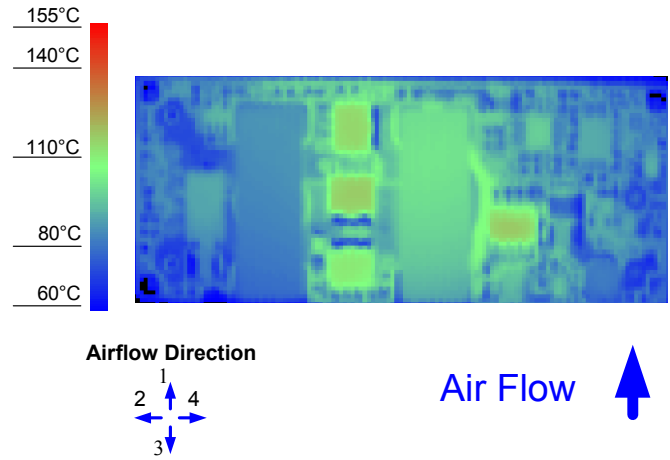
Fig. 10. Thermal Image for Airflow Direction 1 (40A output, 62°C ambient, 200 LFM, Vin = 48V open frame unit)
