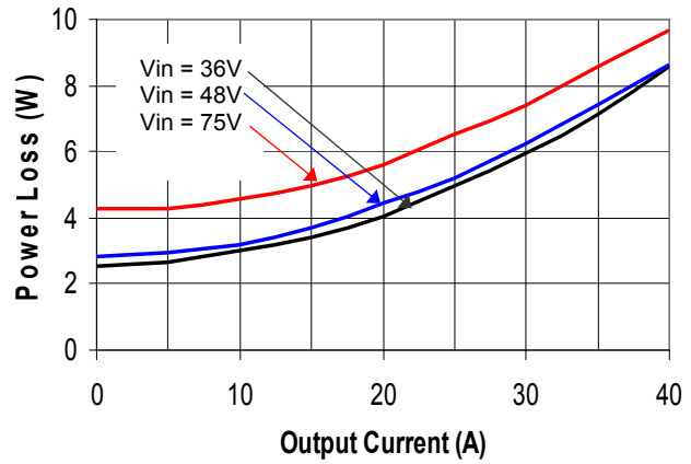
Fig. 2. Power Loss vs. Load Current (25°C)
