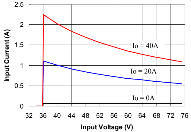
Fig. 4. Input Characteristic
