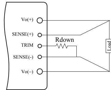
Fig. 14 Circuit to Decrease Output Voltage
