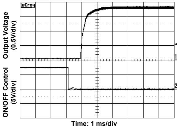
Fig. 3. Start-Up from Enable Control
