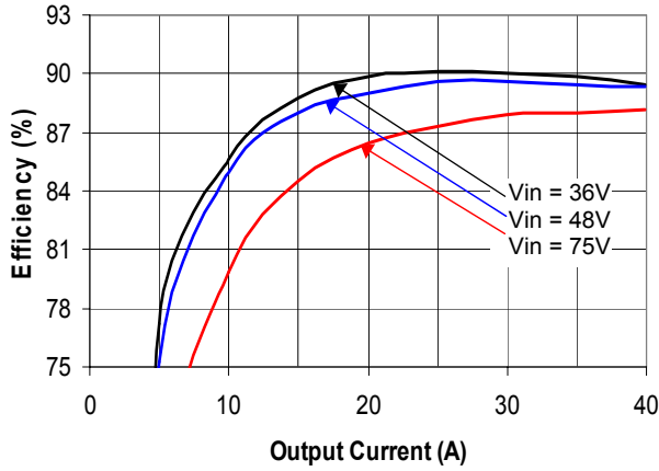
Fig. 1. Efficiency vs. Load Current (25°C)
