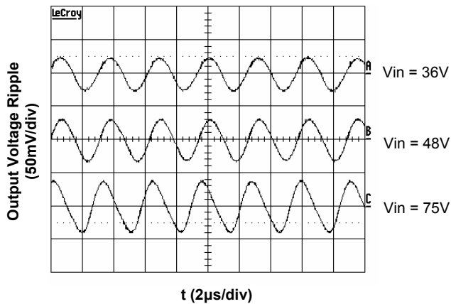
Fig. 5. Output Ripple Voltage at full Load
