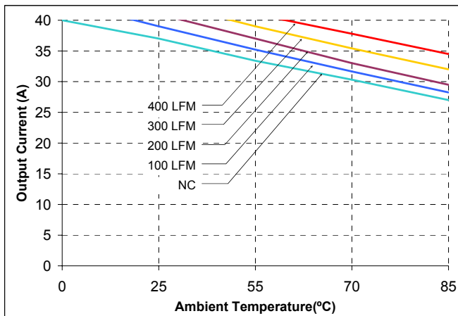
Fig. 9. Current Derating Curve for Airflow Direction 1. (Ref. Fig. 10 for Airflow Direction; Vin = 48V open frame unit )
