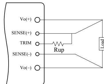
Fig. 15 Circuit to Increase Output Voltage
