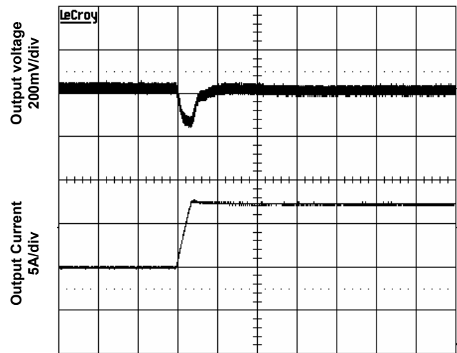
Time - t (200µs/div) Figure 8. Transient Load Response
