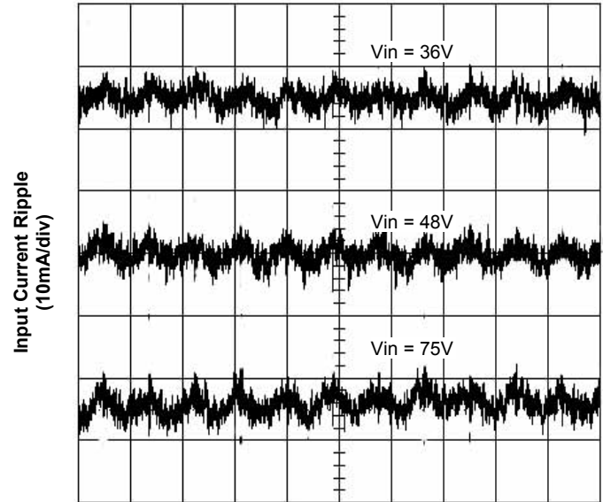
Time - t (5µs/div) Figure 6. Input Reflected Ripple Current at 30A Load
