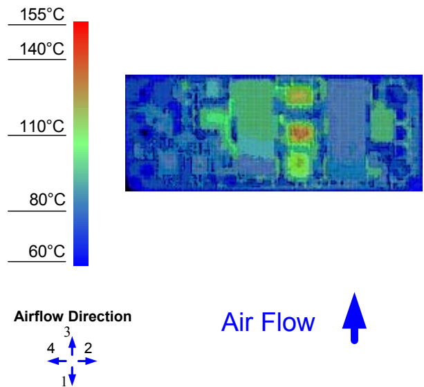
Figure 12. Thermal Image for Airflow Direction 3 (27.5A output, 55°C ambient, 200 LFM, Vin = 48V open frame unit using socket interface)
