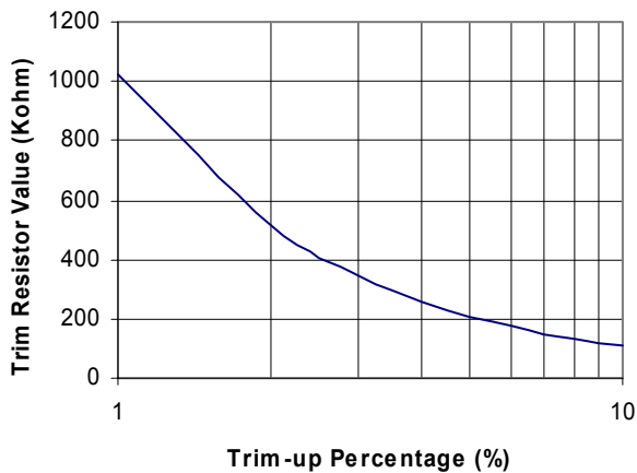
Fig. 19 Trim-Up Resistor Selection
