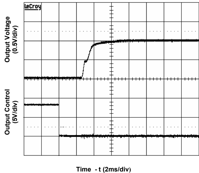
Figure 4. Start-Up from Enable Control Input voltage 48V, Output current 30A
