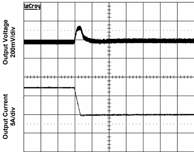
Time - t (200µs/div) Figure 7. Transient Load Response
