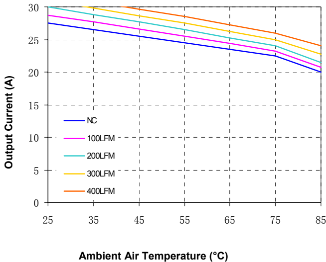
Figure 13. Current Derating Curve for Airflow Direction 2 (Ref. Fig. 14 for Airflow Direction; Vin = 48V open frame unit using socket interface)
