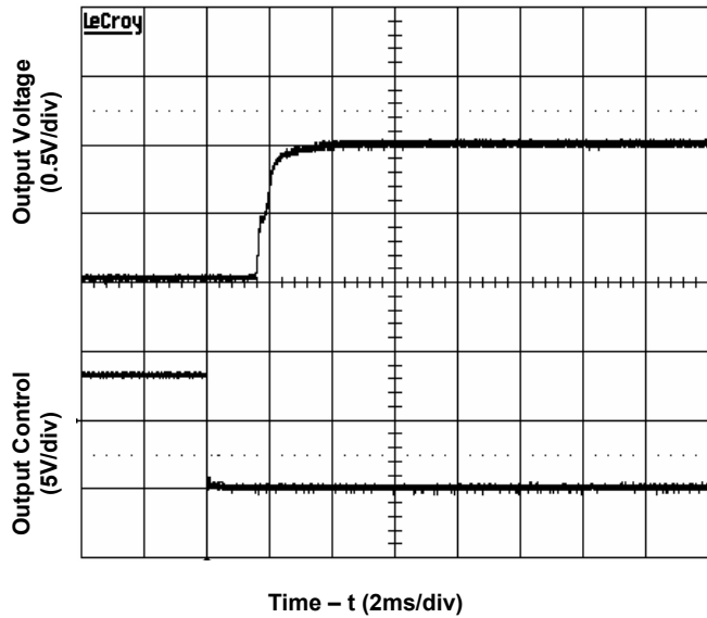
Figure 3. Start-Up from Enable Control Input voltage 48V, Output current 0A
