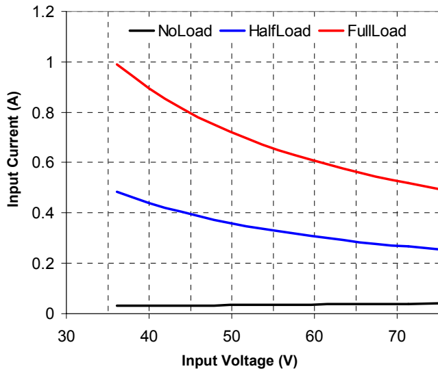
Figure 9. Input Characteristics
