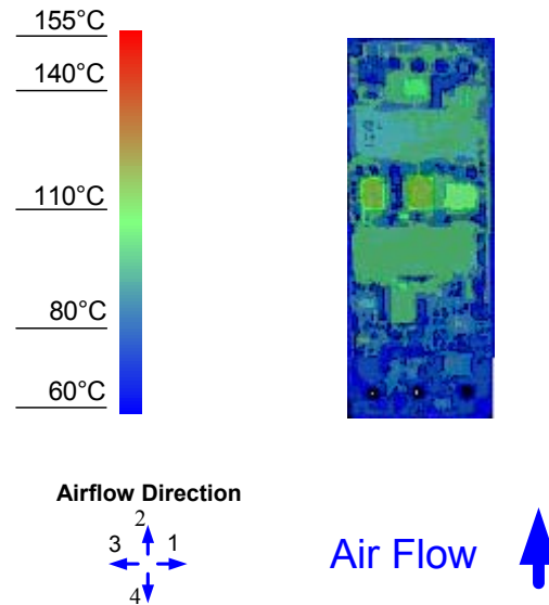
Figure 14. Thermal Image for Airflow Direction 2 (24.8A output, 55°C ambient, 200 LFM, Vin = 48V open frame unit using solder interface)
