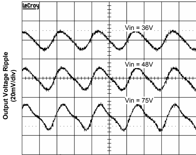
Time - t (2µs/div) Figure 5. Output Ripple Voltage at 30A Load
