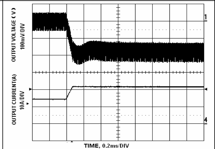
Figure 6 Transient Response to Step Increase (From 50% to 75% Full Load, Vin=48V)
