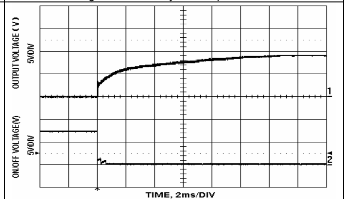
Figure 4 Start-up Using ON/OFF Control with 5000uF Cap. (Vin=48V, Resistive Load (280W))
