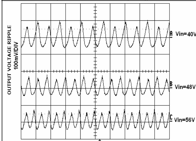
Figure 5 Typical Output Ripple(Po=280W)
