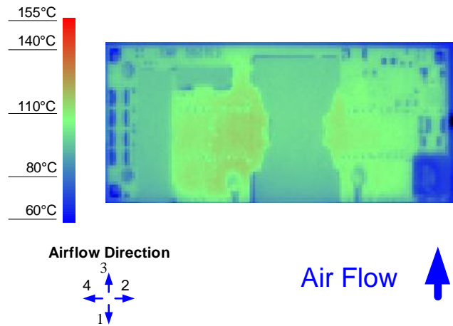
Figure 10 Thermal Image for Airflow Direction 3 (19A output, 55°C ambient, 200 LFM, V_{in} = 48V open frame unit )
