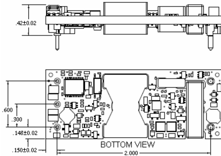
Figure 17 Open Frame Converter
