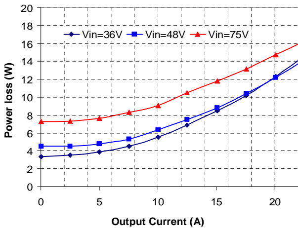
Figure 3 Power loss vs. Output Current
