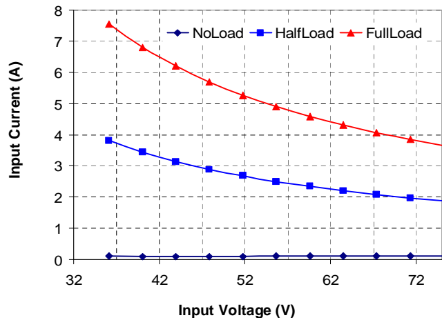
Figure 4 Input Characteristic
