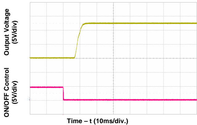
Figure 6 Start-Up from Enable Control Input voltage 48V, Zero load, External Cap.= 47µF
