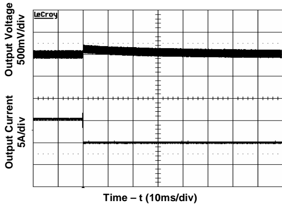
Figure 7 Transient Load Response. Test Cond.: Transient load from 16.5A to 11A, Input voltage 48V, Slew rate 0.1A/ \mu s
