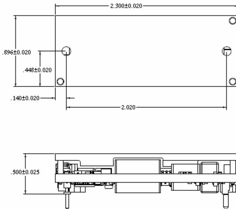
Figure 18 Converter with Baseplate
