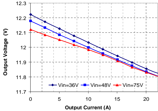
Figure 2 Output Load Regulation (25°C)
