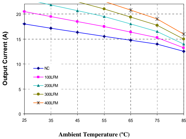
Figure 9 Current Derating Curve for Airflow Direction 3. (Ref. Figure 10 for Airflow Direction; V_{in} = 48V open frame unit )
