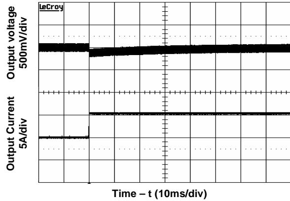
Figure 8 Transient Load Response. Test Cond.: Transient load from 11A to 16.5A, Input voltage 48V, Slew rate 0.1A/ \mu s.
