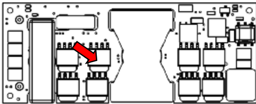
Figure 16 Temperature Monitoring Locations
