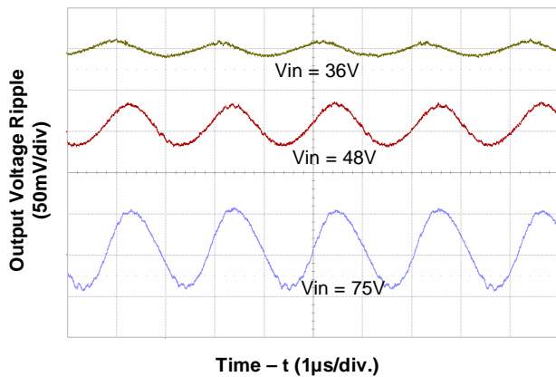
Figure 5 Output Ripple Voltage at Full Load
